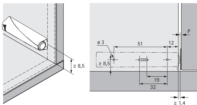
Fitting inset door, for screw on installation, long travel
