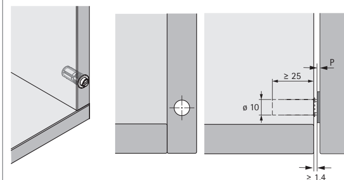
Fitting overlay door, for drill hole installation, lock
