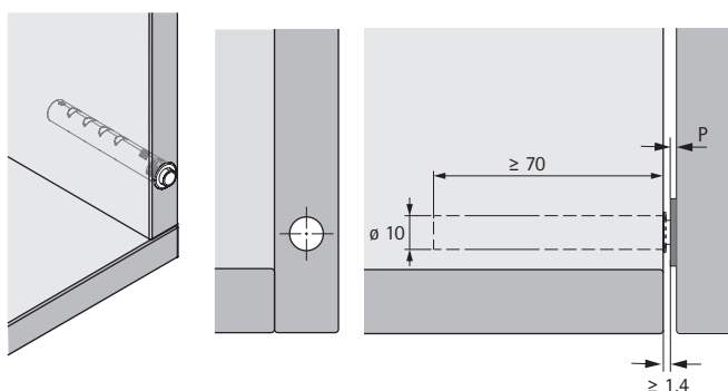
Fitting overlay door, for drill hole installation, long travel
