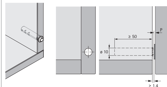
Fitting overlay door, for drill hole installation, short travel
