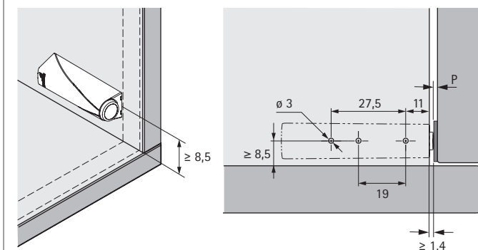
Fitting inset door, for screw on installation, short travel / lock
